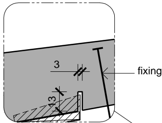
Alternative Sill Flashing For Timber & Concrete
